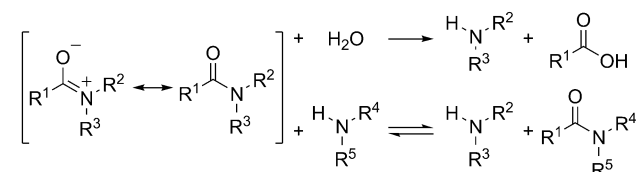
Scheme 1. Deacylation of amides to amines.
